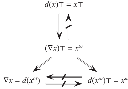
Fig. 2. Relationships between a^\omega and \nabla a .
