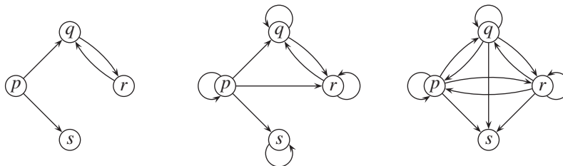
Fig. 1. The relations x , x^* and x^\omega .
