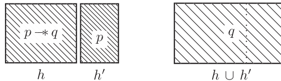
Fig. 1. Separating implication.
