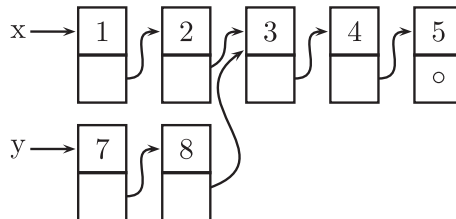
Fig. 2. Two lists with shared cells.
