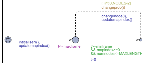
Fig. 6. Uppaal template for the mobility model
