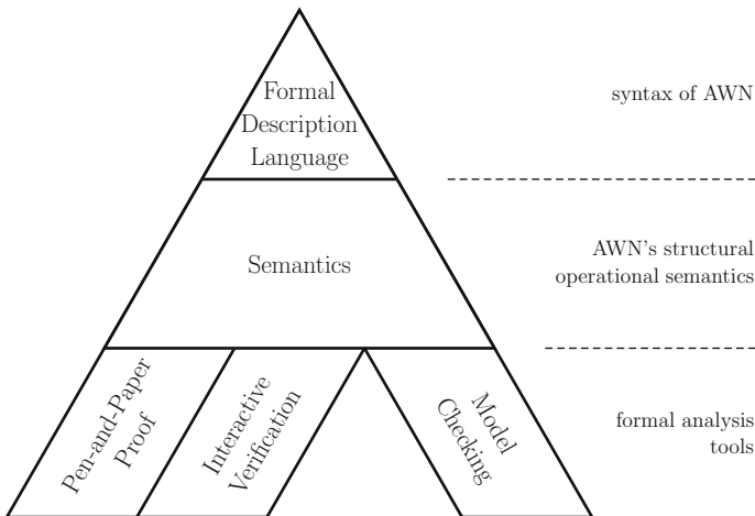
Fig. 3 Different layers of Formal Methods
