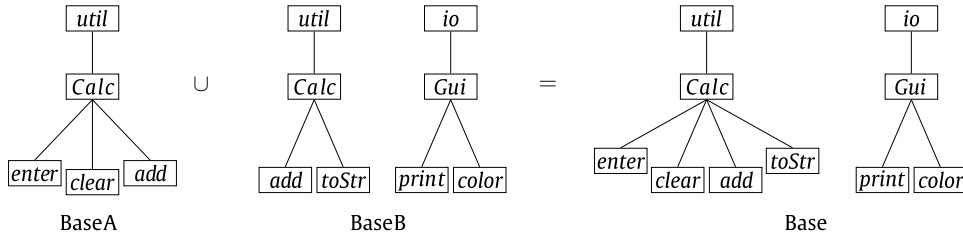
Fig. 2. Superimposition of FSFs.
