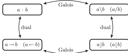
Fig. 1. Relationship between operators of quantales
